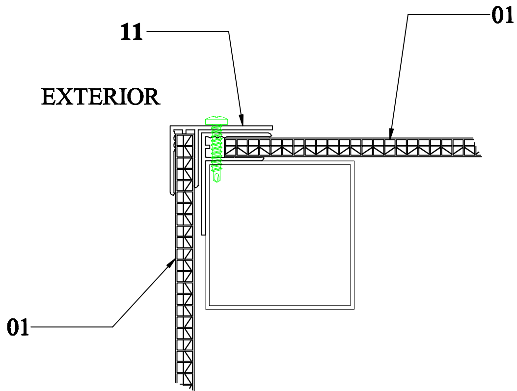
Outside corner
