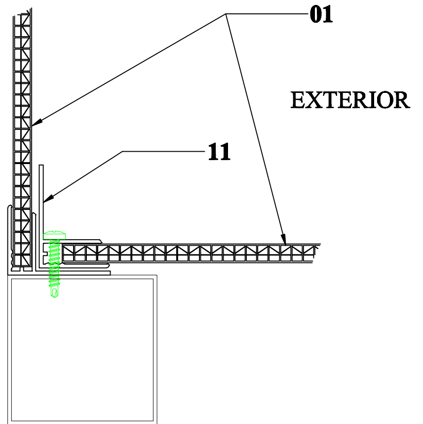
Inside corner
